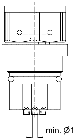
Inner view ( 2 : 1 )
