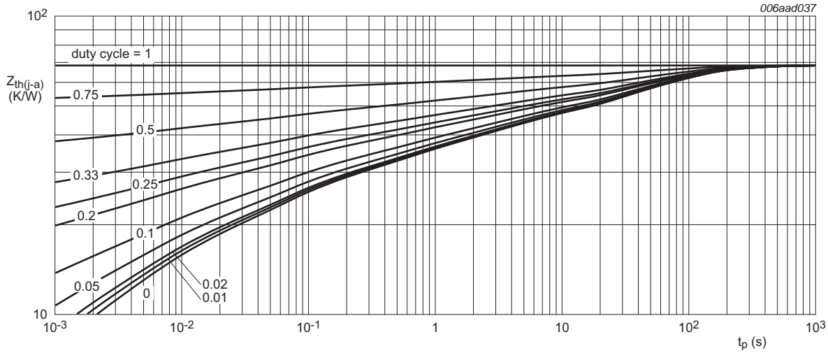
Ceramic PCB, Al 2 O 3 , standard footprint
