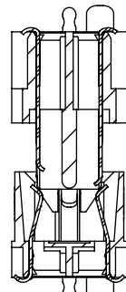
SECTION "E"-"E" SCALE 3 : 1
