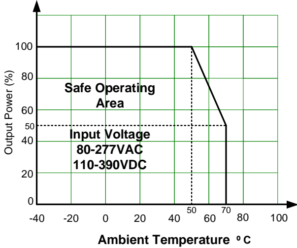
Forced Air Convection
