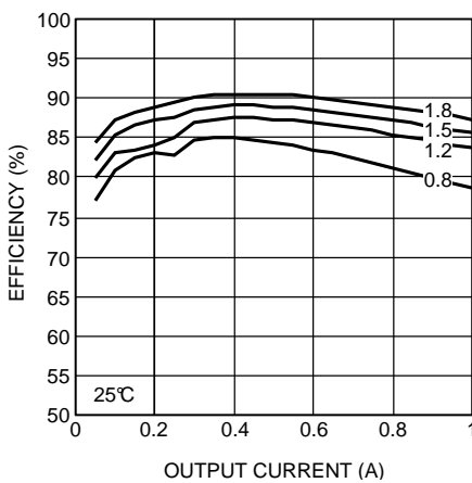
Figure 1. Efficiency 4.5-V Input at 25°C
