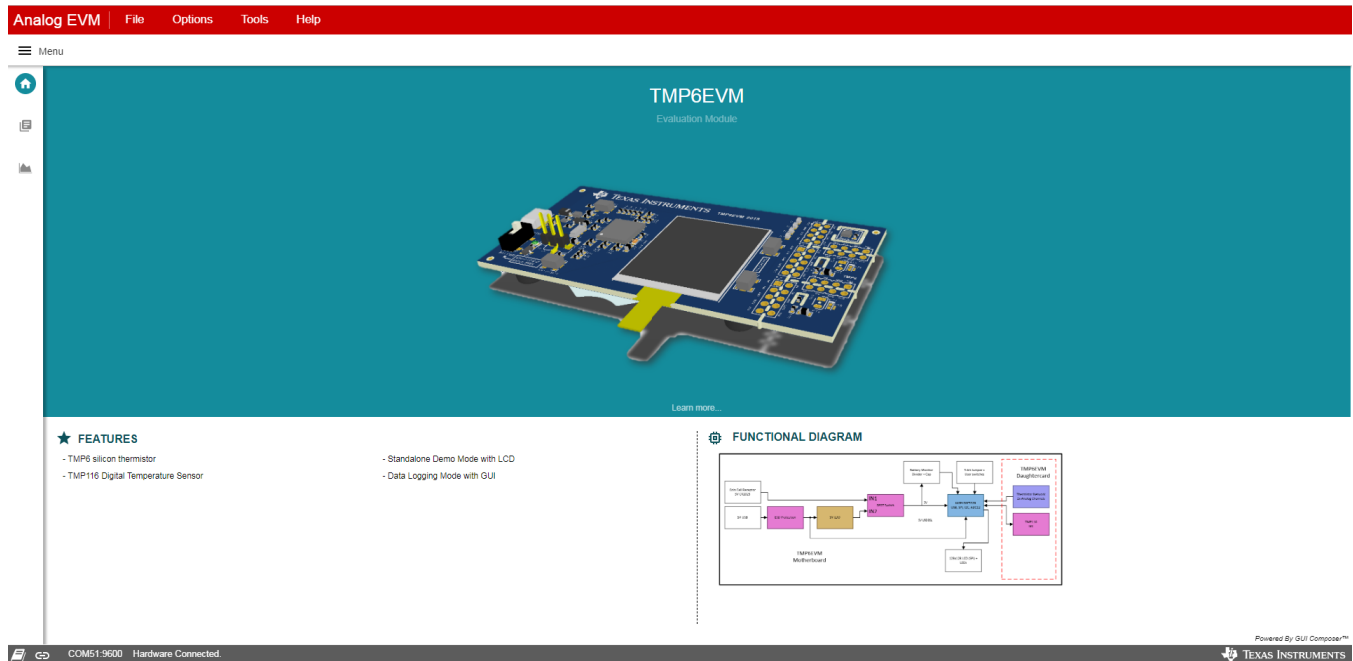
Figure 21. Home Page
