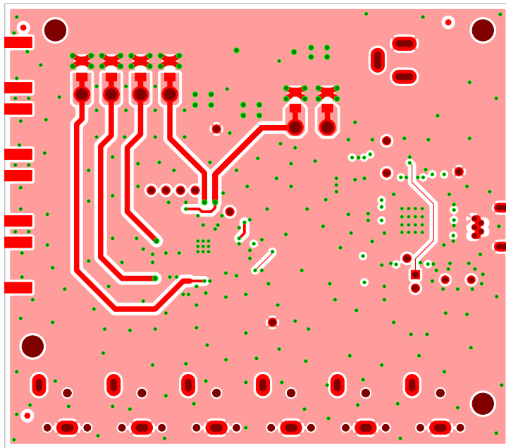
ADV7281AM/ADV7282AMEBZ Eval Board Rev. A (Primary Side View) Secondary Side - Layer 4
