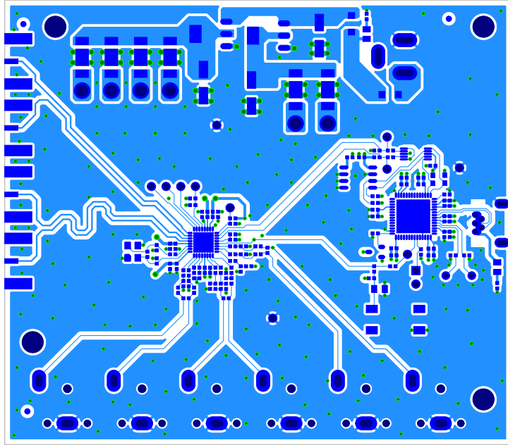
ADV7281AM/ADV7282AMEBZ Eval Board Rev. A (Primary Side View) Primary Side - Layer 1
