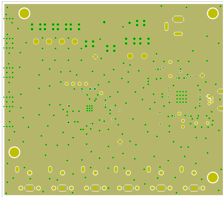
ADV7281AM/ADV7282AMEBZ Eval Board Rev. A (Primary Side View) Ground Plane – Layer 2
