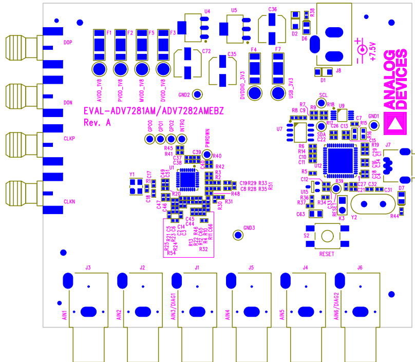
ADV7281AM/ADV7282AMEBZ Eval Board Rev. A (Primary Side View)
