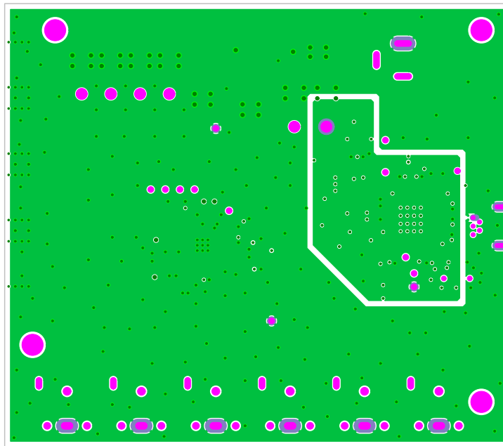
ADV7281AM/ADV7282AMEBZ Eval Board Rev. A (Primary Side View) Power Plane – Layer 3
