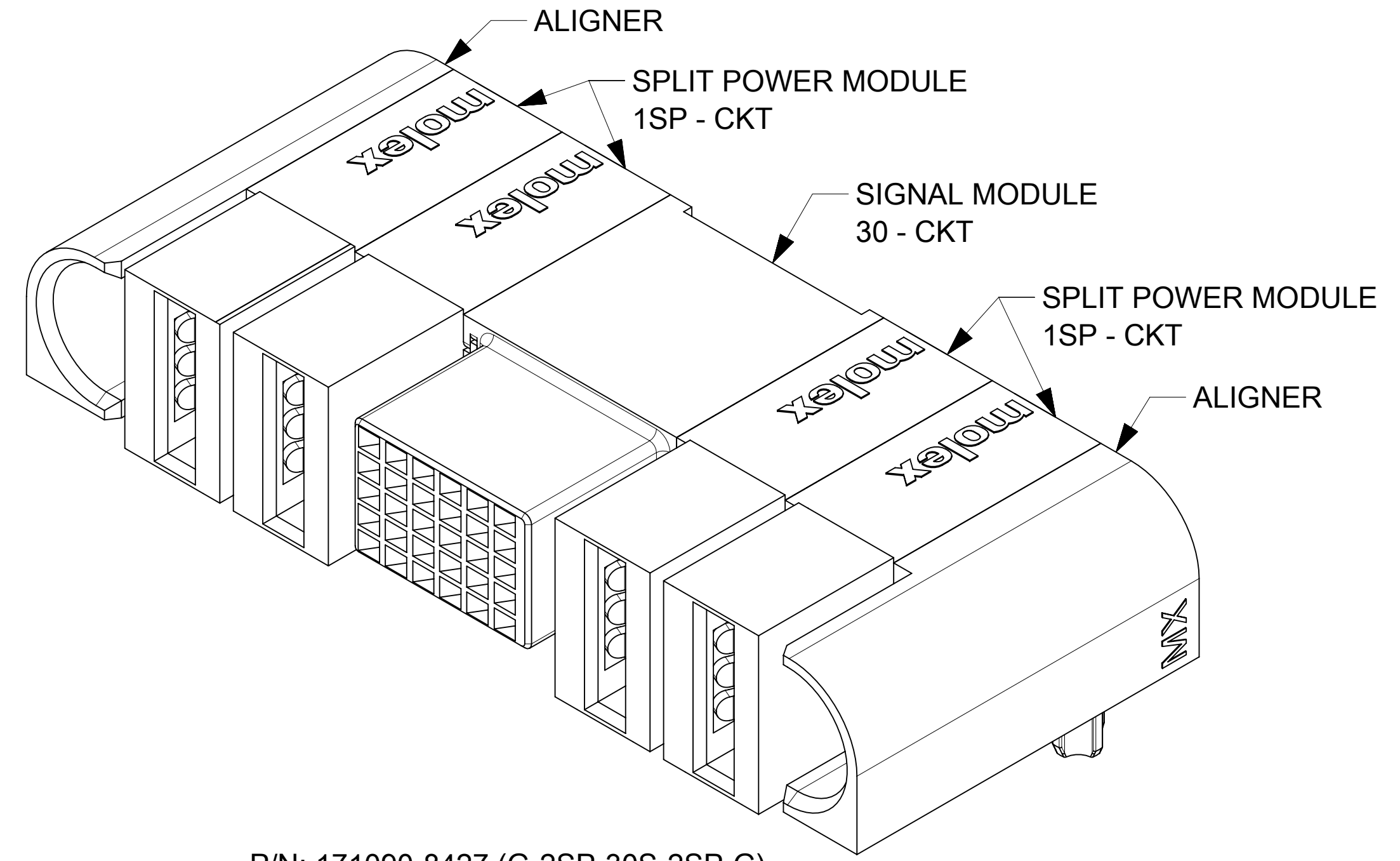
P/N: 171090-8427 (G-2SP-30S-2SP-G)
