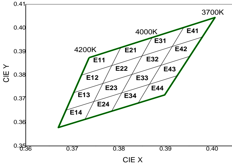
CIE Chromaticity Diagram (Neutral white), T_j=25^\circ\text{C} , I_f=100\text{mA}
