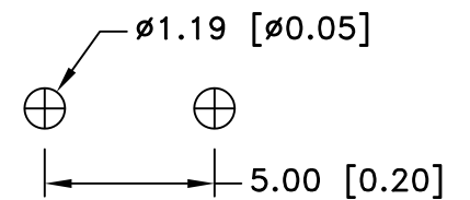
MOUNTING DETAIL
