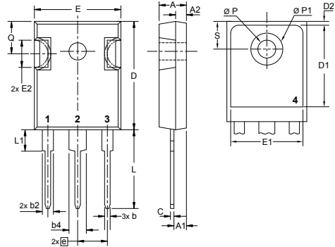
L014a TO-247AD
