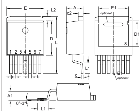
X012b TO-263 (7) middle leg cut Weight = 2.5 g
