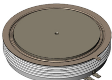
W98 Weight 1.8 kg
