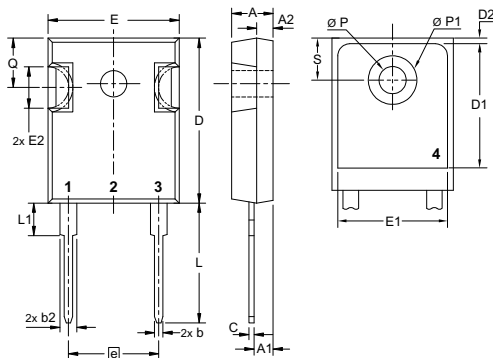
L014b TO-247 AD
