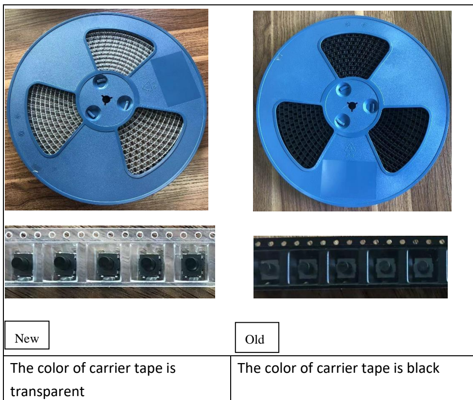
Figure 1: Carrier tape color change
