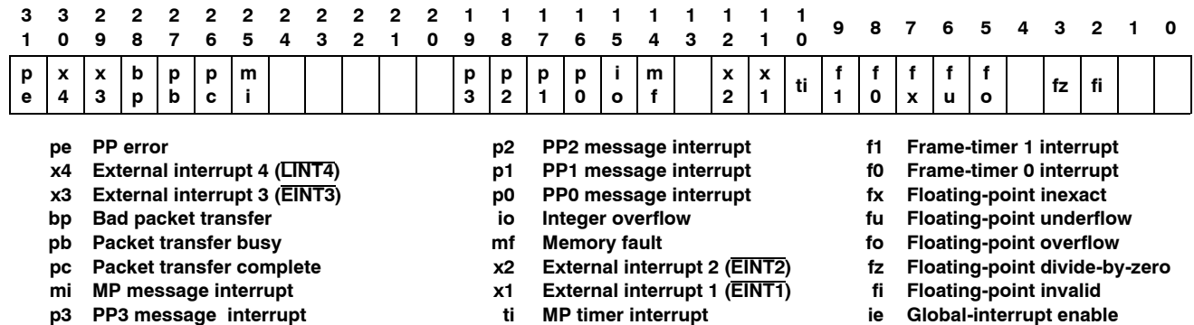
Figure 12. INTPEN Register
