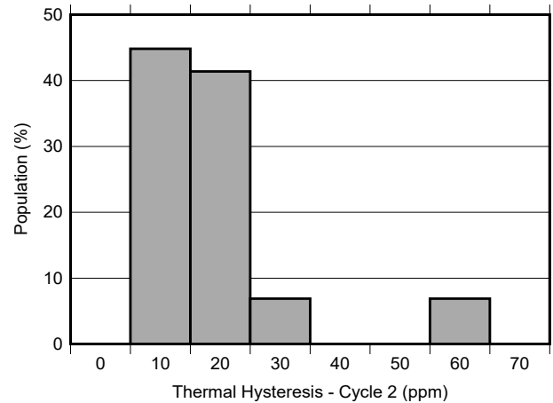
Figure 8-7. Thermal Hysteresis Distribution –40°C to 85°C, Cycle 2
