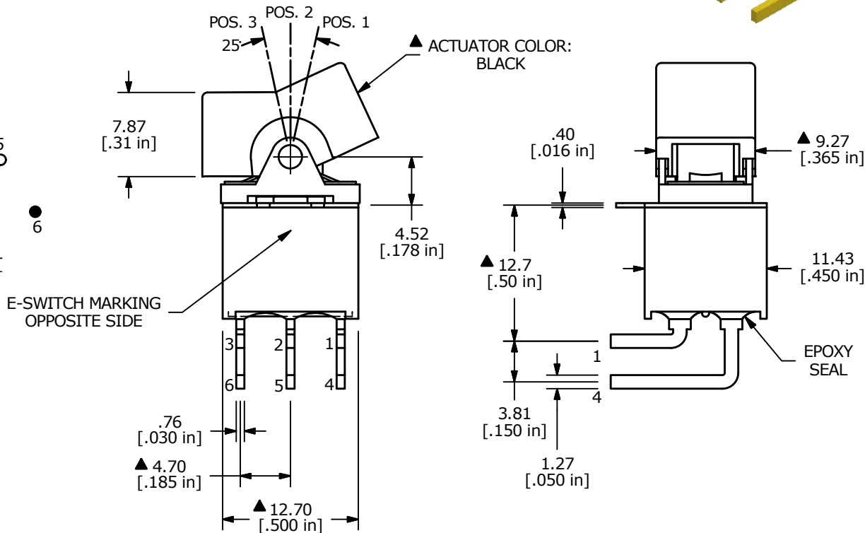
CIRCUIT: DPDT
