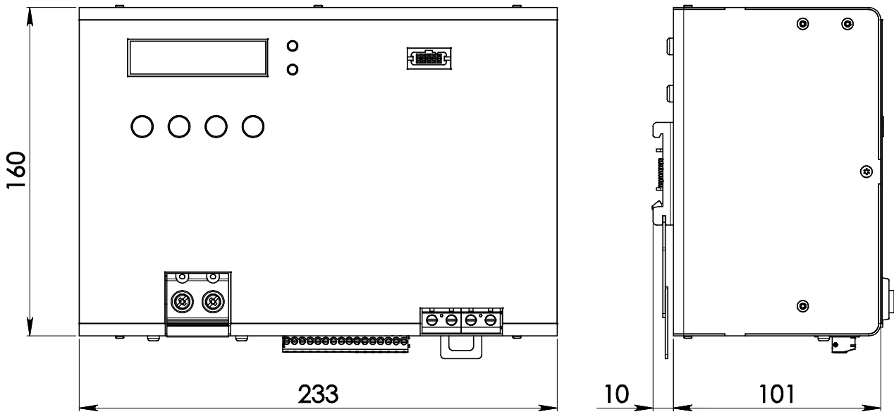
Figure 2. Mechanical Drawing
