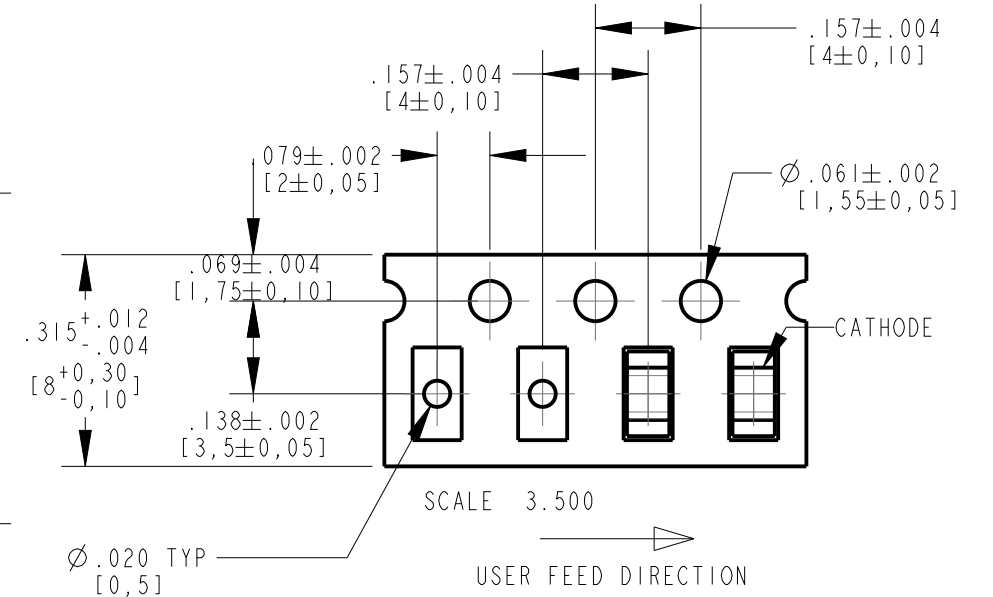
PACKAGE DIMENSIONS OF TAPE AND REEL
