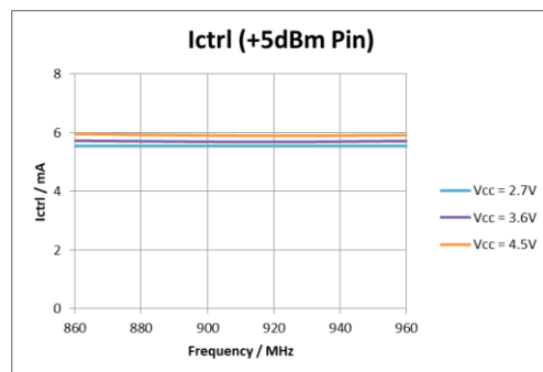
Figure 23: Ictrl (+5 dBm Pin)
