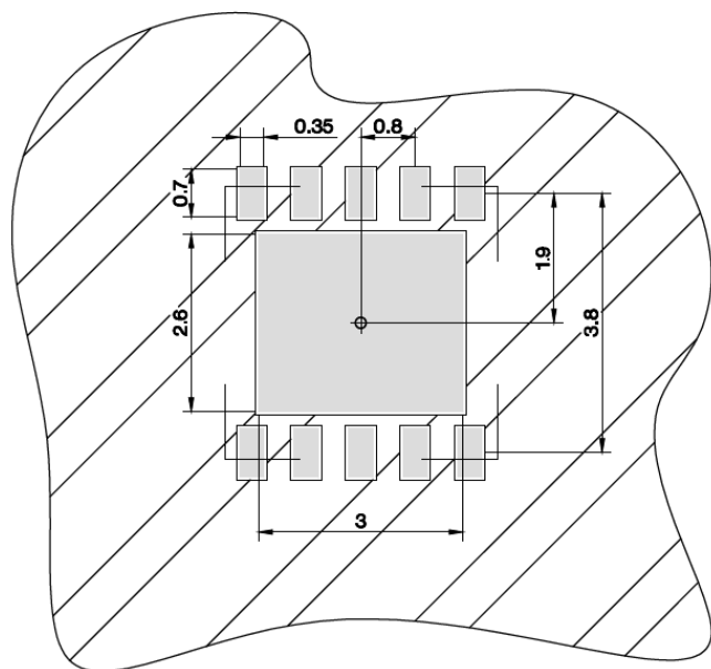
PG-WSON-10-1: Boardpads & Apertures
