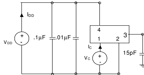
Figure 2. Typical Output Test Conditions (25±5°C)
