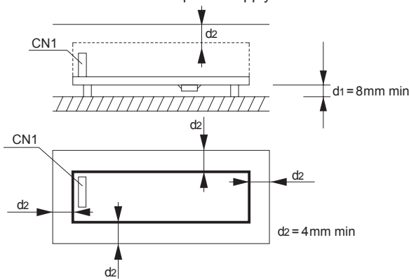
Fig.3.1 Installation method
