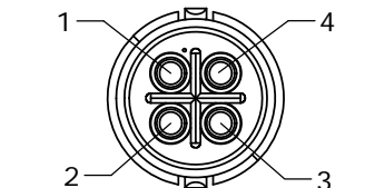
WIRE VIEW 6380-4PG-3XXW SHOWN
