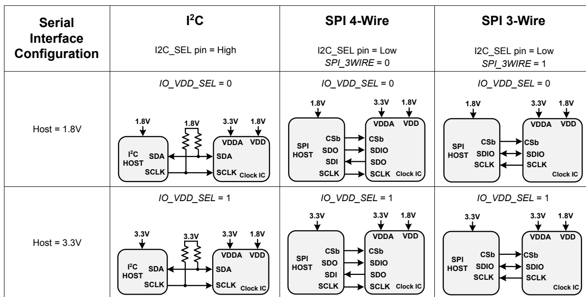
Figure 6.1. I 2 C/SPI Device Connectivity Configurations
