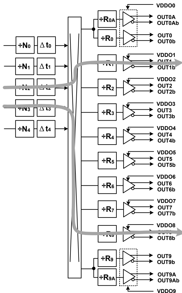
Figure 4.4. Example of Independently-Configurable Path Delays
