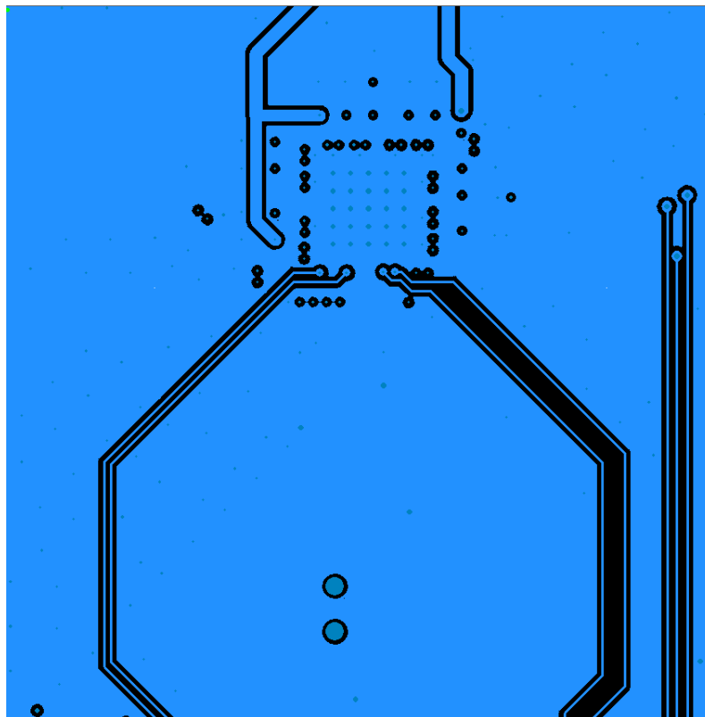
Figure 9.4. External XO: Internal Power Plane (Layer 4)
