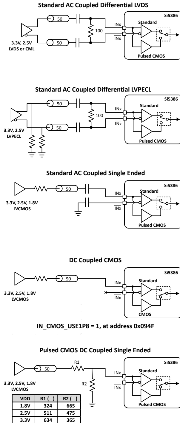
Figure 3.1. Input Termination for Standard and CMOS Inputs
