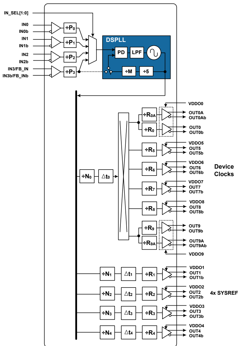
Figure 1.1. Si5386 Block Diagram
