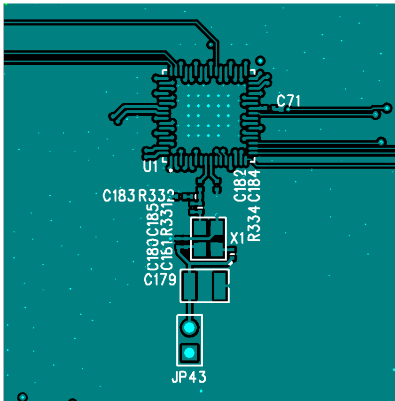
Figure 9.1. External XO: Si5386 Device and XO Layout Recommendations, Top Layer (Layer 1)
