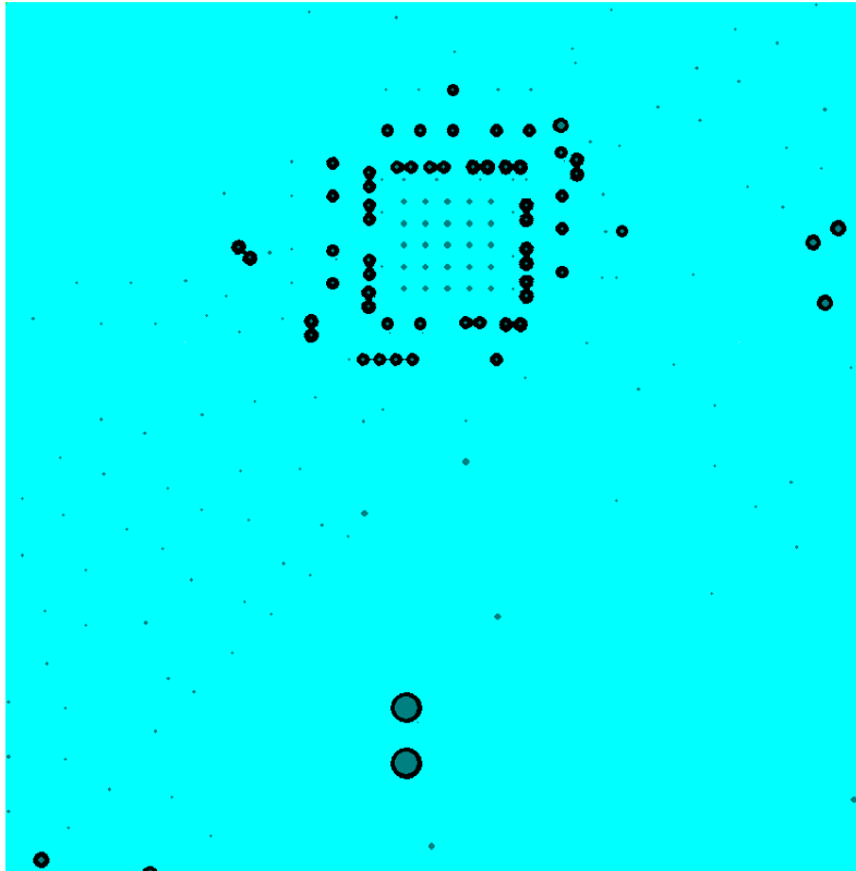
Figure 9.3. External XO: Internal Ground Plane (Layer 3)
