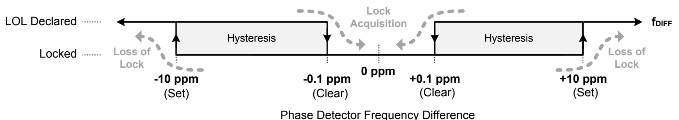
Figure 3.7. Example of LOL Set and Clear Thresholds
