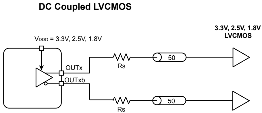
Figure 4.3. LVC MOS Output Terminations
