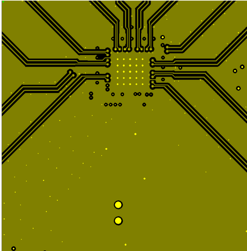
Figure 9.7. External XO: Output Clocks (Layer 7)
