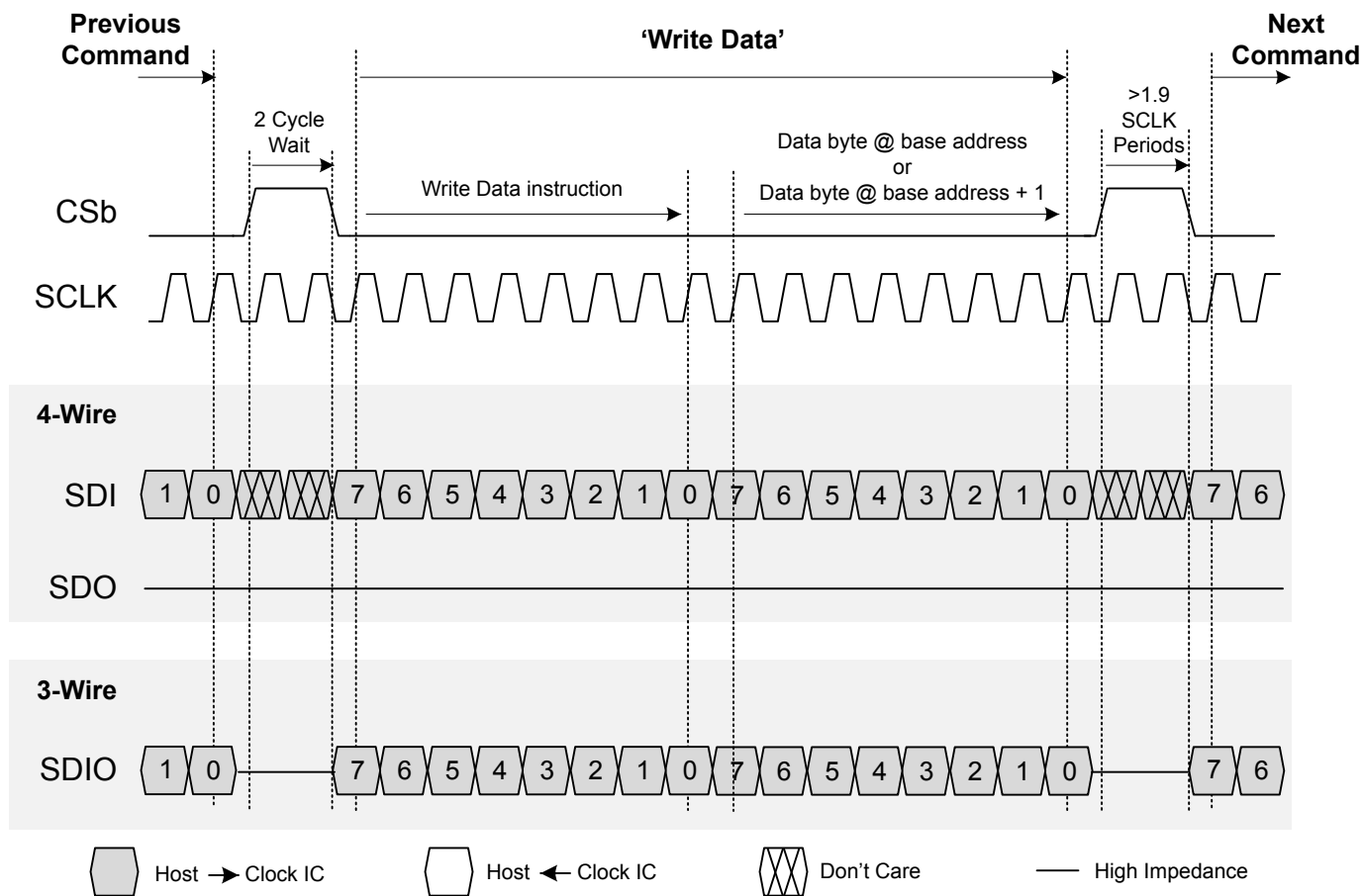
Figure 6.10. SPI "Write Data" and "Write Data + Address Increment" Instruction Timing
