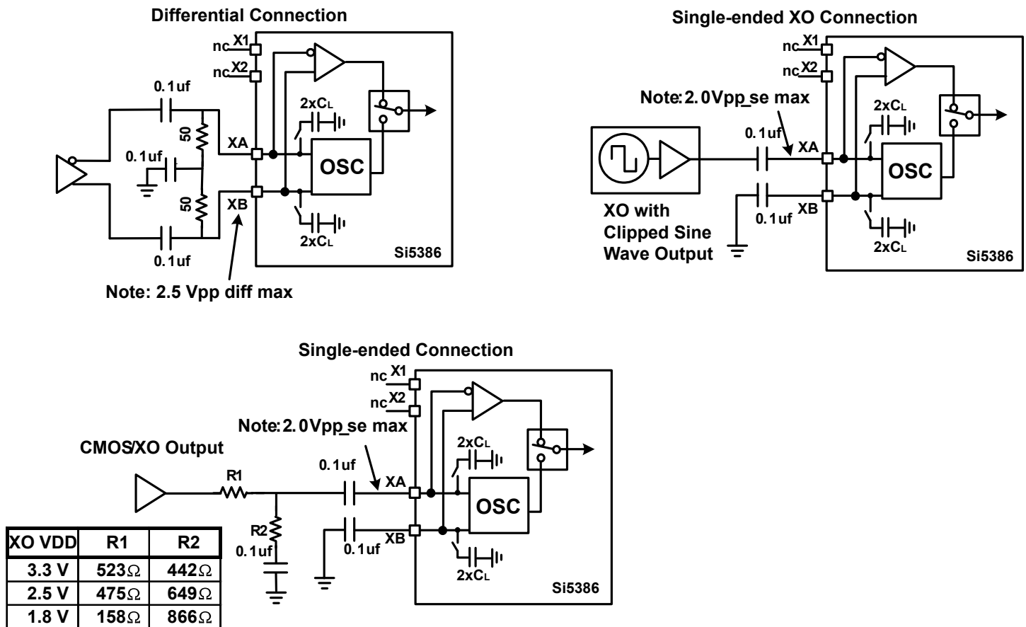
Figure 8.1. XAXB External Reference Clock Connection Options
