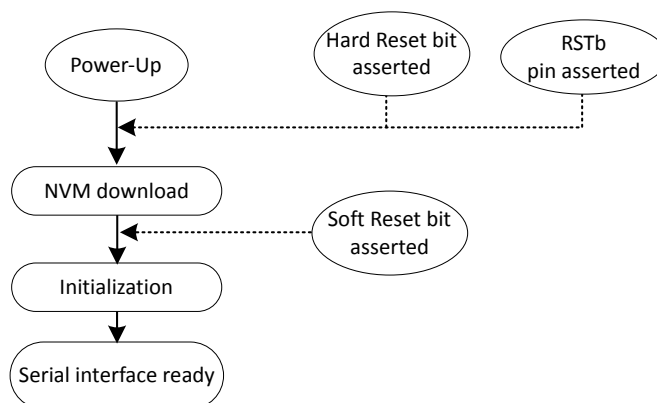
Figure 2.2. Initialization from Hard Reset and Soft Reset
