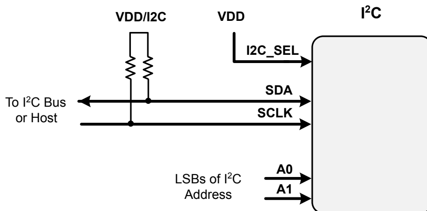
Figure 6.2. Si5386 I 2 C Configuration
