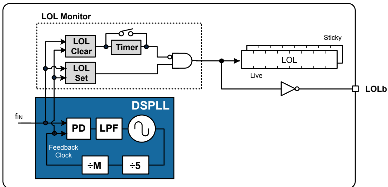
Figure 3.6. Si5386 LOL Status Indicator
