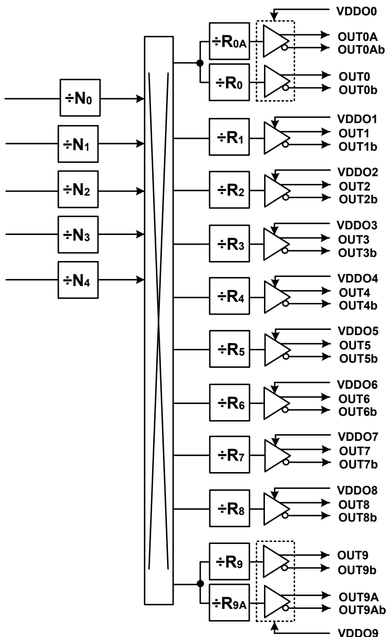
Figure 4.1. N Divider to Output Driver Crosspoint
