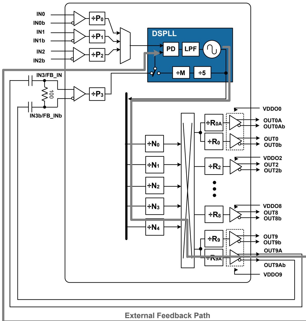
Figure 5.1. Si5386 Zero Delay Mode (ZDM) Setup
