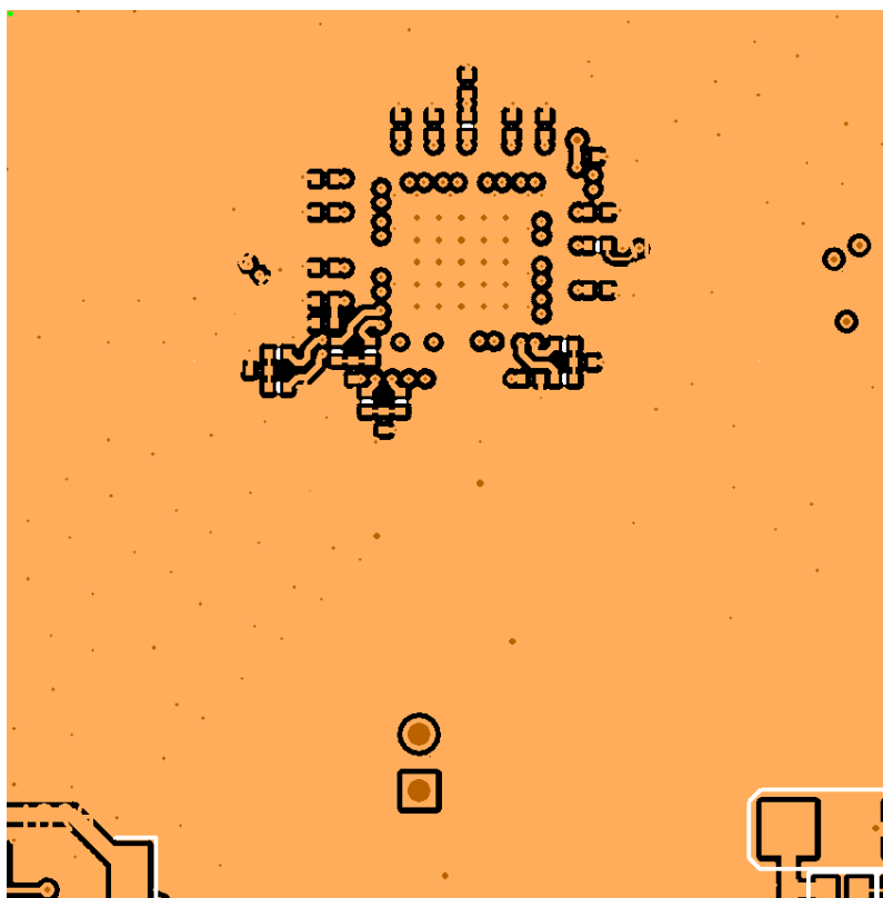
Figure 9.8. External XO: Bottom Layer Ground Flooded (Layer 8)
