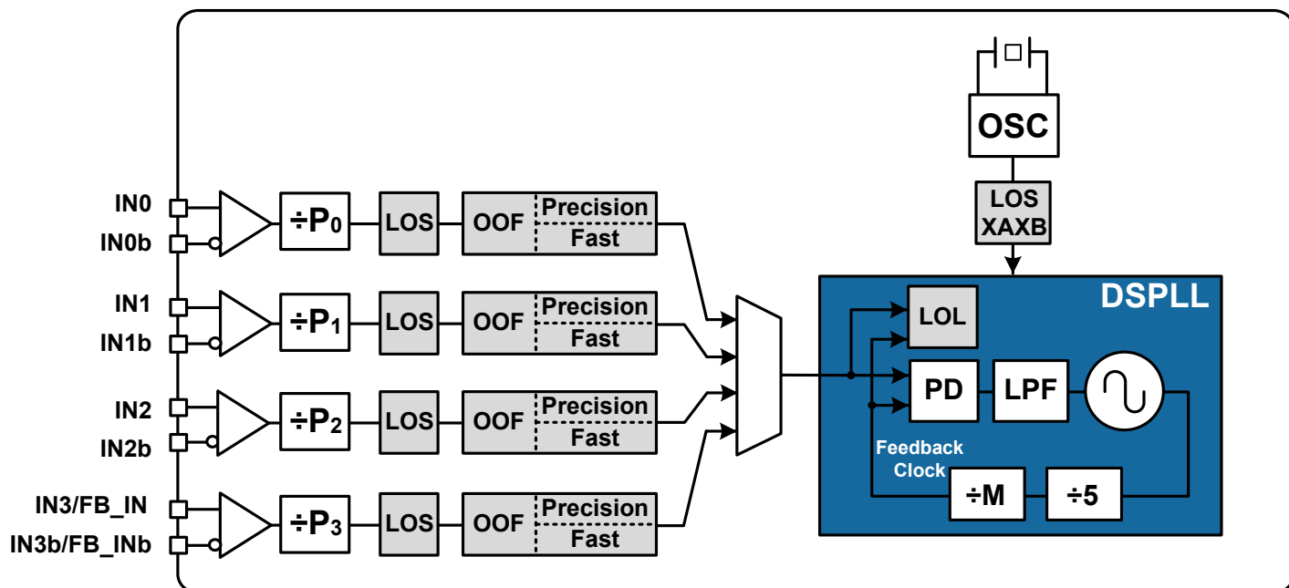
Figure 3.2. Si5386 Fault Monitors
