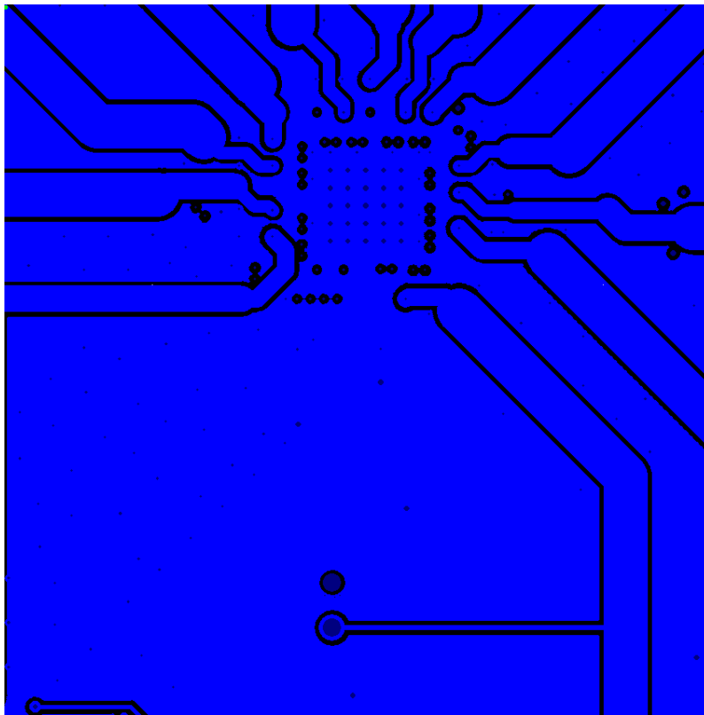
Figure 9.5. External XO: Internal Power Plane (Layer 5)
