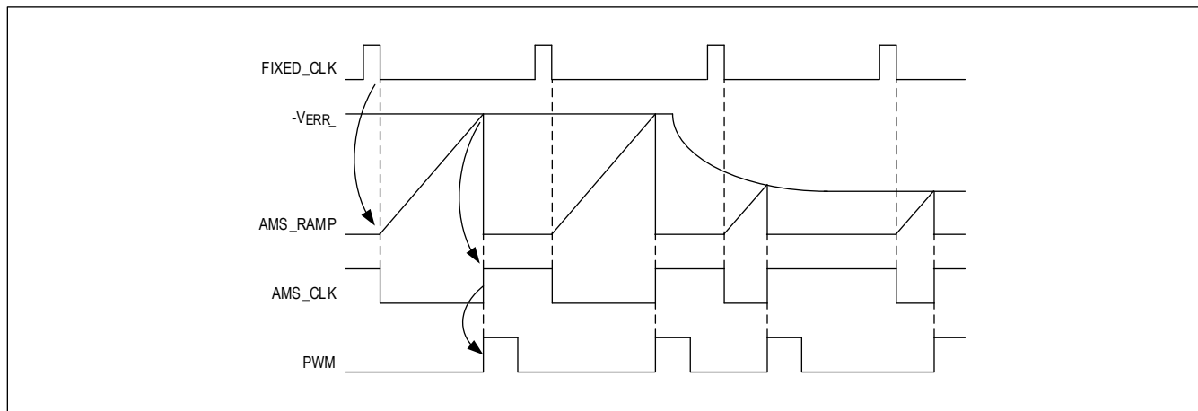
Figure 2. AMS Operation
