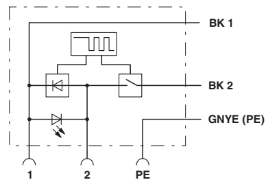
Contact assignment of the valve plug
