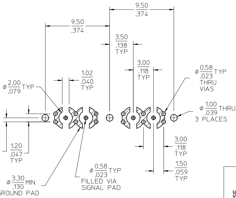
PCB LAYOUT
