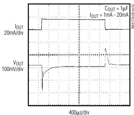
LOAD TRANSIENT
