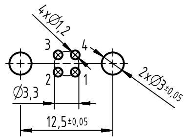
panel cut-out
