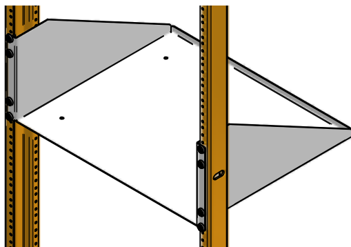
COMPLETE ASSEMBLY
