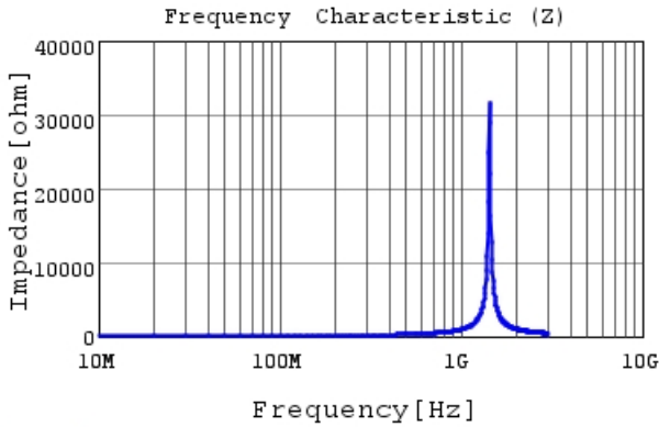
LQG15WZ82NJ02 |Z|
