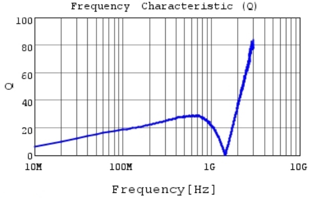
LQG15WZ82NJ02 Q
