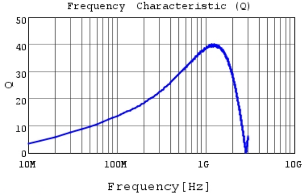
LQG15WZ22NG02 Q
