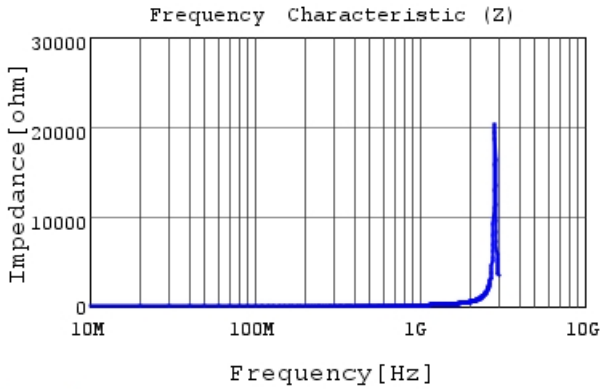
LQG15WZ22NG02 |Z|
