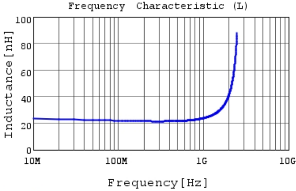
LQG15WZ22NG02 L
