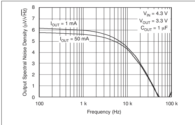
Figure 6-19. Output Spectral Noise Density vs Frequency for Legacy Chip
