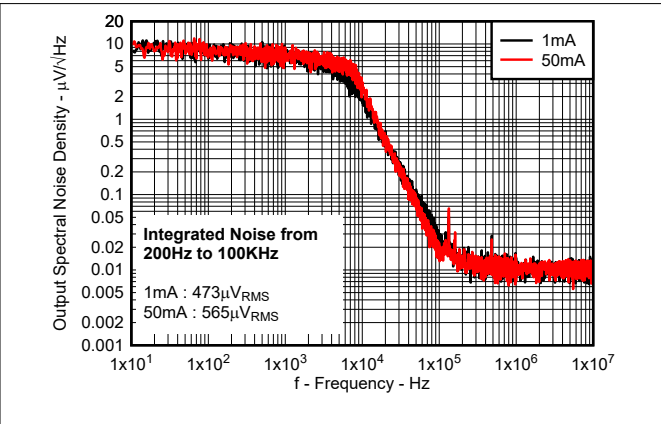
Figure 6-20. Output Spectral Noise Density vs Frequency for New Chip
