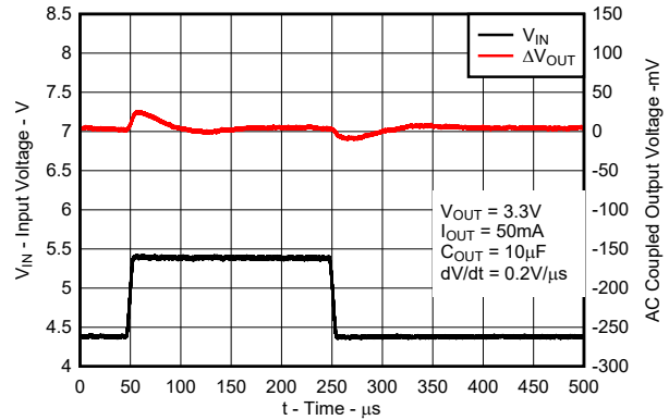
Figure 8-6. Line Transient Response for New Chip
