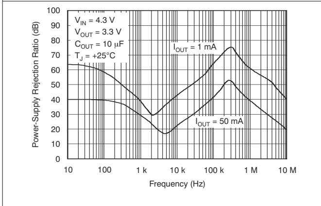
Figure 6-21. Power-Supply Ripple Rejection vs Frequency for Legacy Chip
