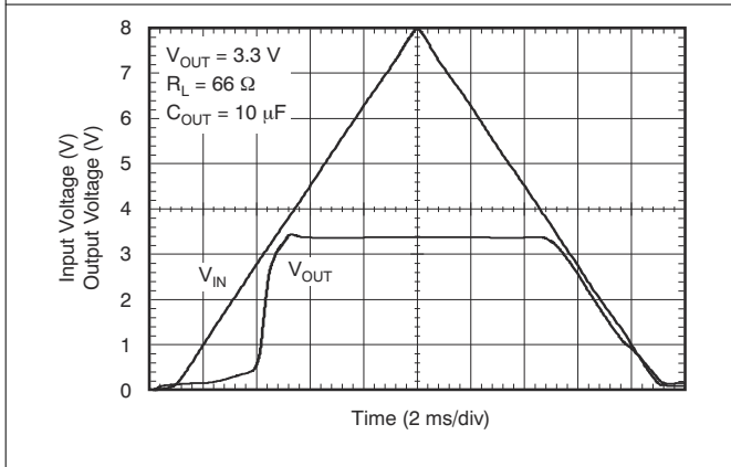
Figure 6-23. Power-Up, Power-Down for Legacy Chip
