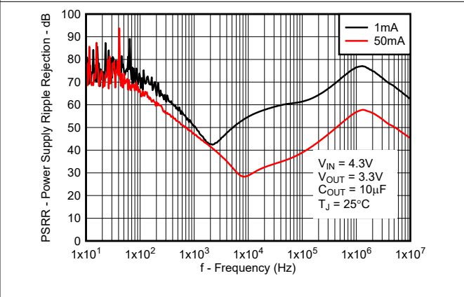
Figure 6-22. Power-Supply Ripple Rejection vs Frequency for New Chip
