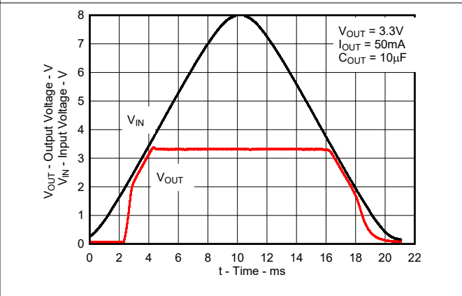
Figure 6-24. Power-Up, Power-Down for New Chip
