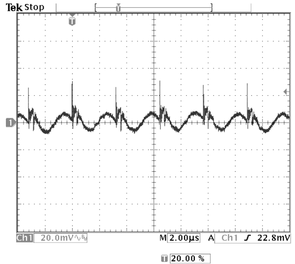
Fig-1.0V-5: Output voltage ripple (20mV/div.) for V_{out}=1.0V at full rated load current into a resistive load with external capacitance 47\mu F \times 2 ceramic + 1uF ceramic at V_{in}=12.0V . Time scale: 2 us/div
