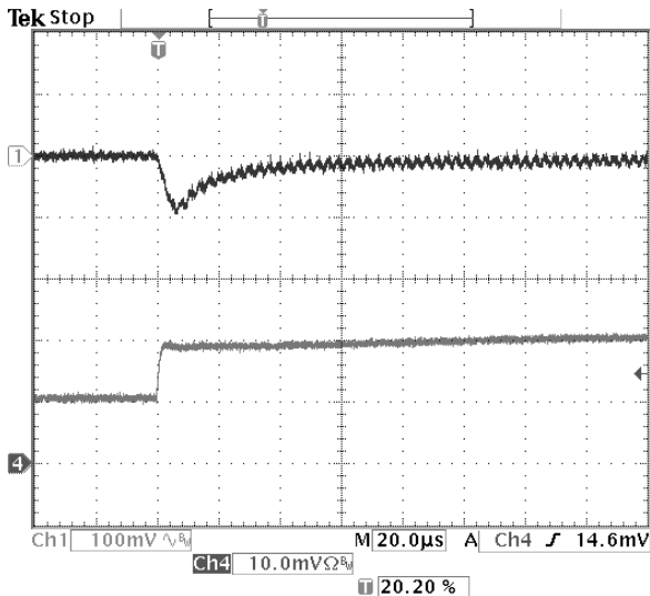
Fig-1.0V-6: Output voltage response for V_{out}=1.0V to positive load current step-change from 5A to 10A with slew rate of 5A/us at V_{in}=12.0V . C_o=47\mu F \times 2 ceramic. Top trace: output voltage (100mV/div.) Bottom trace: load current (5A/div.) Time scale: 20us/div.
