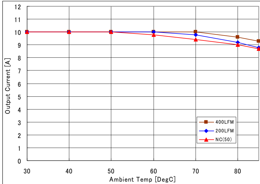
Fig-1.2V-1: Available load current vs. ambient temperature and airflow rates for Vout=1.2V with Vin=12.0V. Maximum component temperature \leq 120^{\circ}\text{C}
