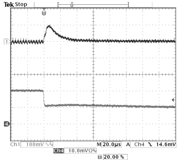
Fig-1.2V-7: Output voltage response for V_{out}=1.2V to positive load current step-change from 10A to 5A with slew rate of -5A/\mu s at V_{in}=12.0V . C_o=47\mu F \times 2 ceramic. Top trace: output voltage (100mV/div.) Bottom trace: load current (5A/div.) Time scale: 20us/div.
