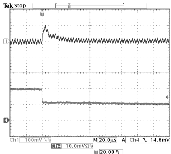
Fig-5.0V-7: Output voltage response for V_{out}=5.0V to positive load current step-change from 10A to 5A with slew rate of -5A/\mu s at V_{in}=12.0V . C_o=47\mu F \times 2 ceramic. Top trace: output voltage (100mV/div.) Bottom trace: load current (5A/div.) Time scale: 20us/div.
