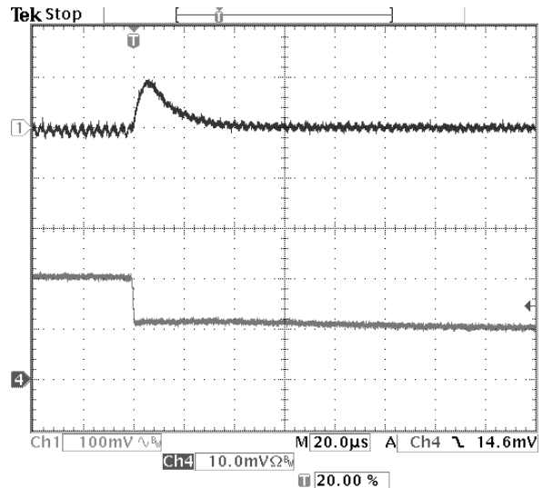
Fig-1.5V-7: Output voltage response for V_{out}=1.5V to positive load current step-change from 10A to 5A with slew rate of -5A/\mu s at V_{in}=12.0V . C_o=47\mu F \times 2 ceramic. Top trace: output voltage (100mV/div.) Bottom trace: load current (5A/div.) Time scale: 20us/div.
