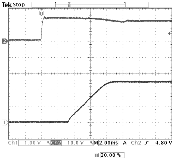
Fig-2.5V-4: Turn-on transient for V_{out}=2.5V with application of V_{in} at full rated load current (resistive) and 47\mu F \times 2 external capacitance at V_{in}=12.0V . Top trace: V_{in} (10V/div.) Bottom trace: output voltage (1V/div.) Time scale: 2 ms/div.
