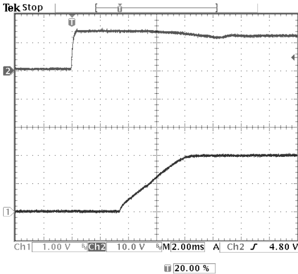
Fig-2.0V-4: Turn-on transient for V_{out}=2.0V with application of V_{in} at full rated load current (resistive) and 47\mu F \times 2 external capacitance at V_{in}=12.0V . Top trace: V_{in} (10V/div.) Bottom trace: output voltage (1V/div.) Time scale: 2 ms/div.
