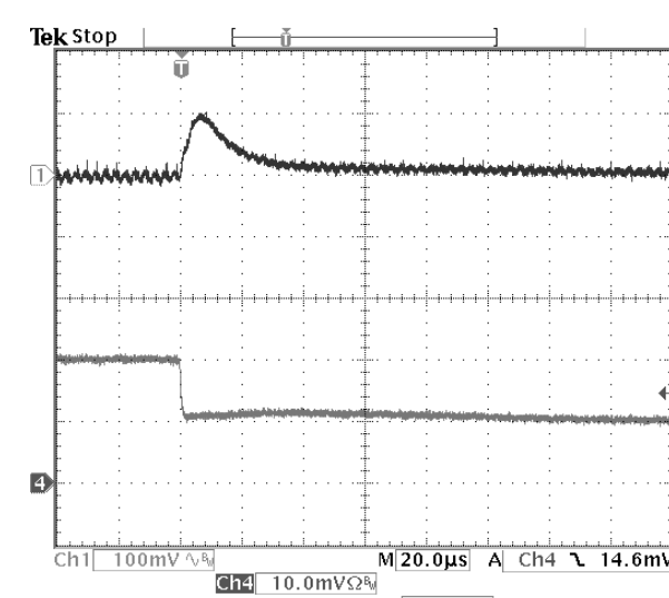
Fig-1.0V-7: Output voltage response for V_{out}=1.0V to positive load current step-change from 10A to 5A with slew rate of -5A/us at V_{in}=12.0V . C_o=47\mu F \times 2 ceramic. Top trace: output voltage (100mV/div.) Bottom trace: load current (5A/div.) Time scale: 20us/div.
