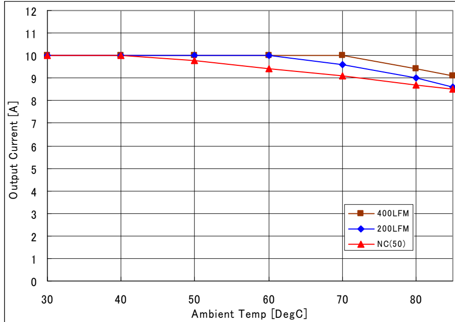
Fig-2.0V-1: Available load current vs. ambient temperature and airflow rates for Vout=2.0V with Vin=12.0V. Maximum component temperature \leq 120^{\circ}\text{C}
