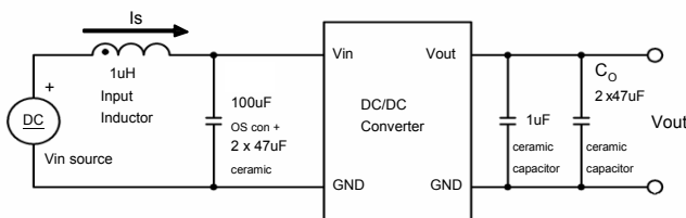
Fig. G: Test setup for measuring input reflected ripple current
