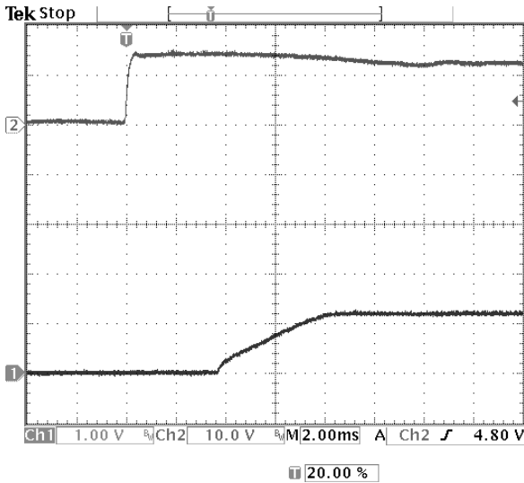
Fig-1.2V-4: Turn-on transient for V_{out}=1.2V with application of V_{in} at full rated load current (resistive) and 47\mu F \times 2 external capacitance at V_{in}=12.0V . Top trace: V_{in} (10V/div.) Bottom trace: output voltage (1V/div.) Time scale: 2 ms/div.
