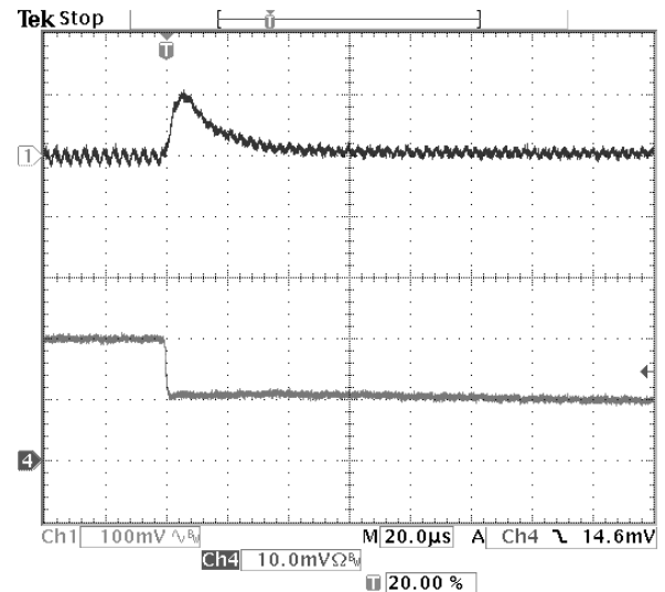
Fig-2.0V-7: Output voltage response for V_{out}=2.0V to positive load current step-change from 10A to 5A with slew rate of -5A/us at V_{in}=12.0V . C_o=47\mu F \times 2 ceramic. Top trace: output voltage (100mV/div.) Bottom trace: load current (5A/div.) Time scale: 20us/div.
