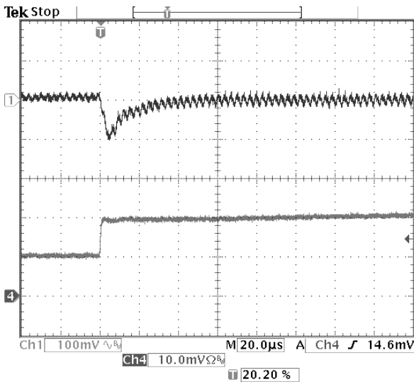
Fig-2.5V-6: Output voltage response for V_{out}=2.5V to positive load current step-change from 5A to 10A with slew rate of 5A/us at V_{in}=12.0V . C_o=47\mu F \times 2 ceramic. Top trace: output voltage (100mV/div.) Bottom trace: load current (5A/div.) Time scale: 20us/div.
