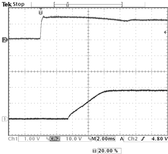
Fig-1.8V-4: Turn-on transient for V_{out}=1.8V with application of V_{in} at full rated load current (resistive) and 47\mu F \times 2 external capacitance at V_{in}=12.0V . Top trace: V_{in} (10V/div.) Bottom trace: output voltage (1V/div.) Time scale: 2 ms/div.
