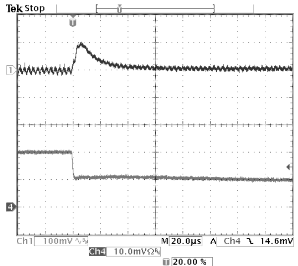
Fig-1.8V-7: Output voltage response for V_{out}=1.8V to positive load current step-change from 10A to 5A with slew rate of -5A/us at V_{in}=12.0V . C_o=47\mu F \times 2 ceramic. Top trace: output voltage (100mV/div.) Bottom trace: load current (5A/div.) Time scale: 20us/div.
