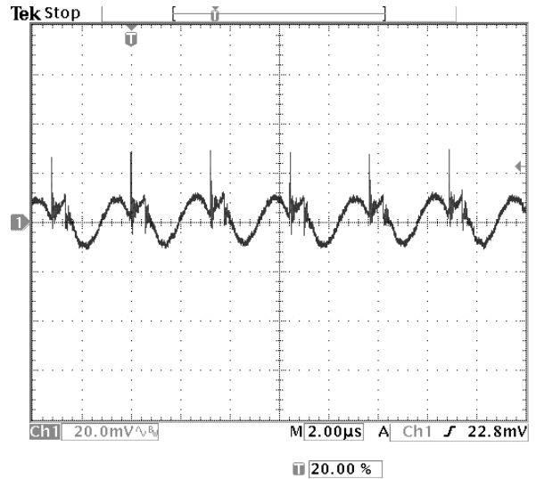
Fig-1.8V-5: Output voltage ripple (20mV/div.) for V_{out}=1.8V at full rated load current into a resistive load with external capacitance 47\mu F \times 2 ceramic + 1uF ceramic at V_{in}=12.0V . Time scale: 2 us/div
