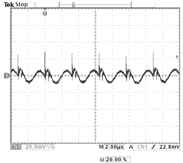
Fig-1.2V-5: Output voltage ripple (20mV/div.) for V_{out}=1.2V at full rated load current into a resistive load with external capacitance 47\mu F \times 2 ceramic + 1\mu F ceramic at V_{in}=12.0V . Time scale: 2 us/div
