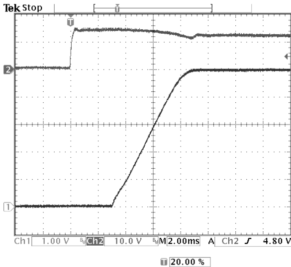
Fig-5.0V-4: Turn-on transient for V_{out}=5.0V with application of V_{in} at full rated load current (resistive) and 47\mu F \times 2 external capacitance at V_{in}=12.0V . Top trace: V_{in} (10V/div.) Bottom trace: output voltage (1V/div.) Time scale: 2 ms/div.
