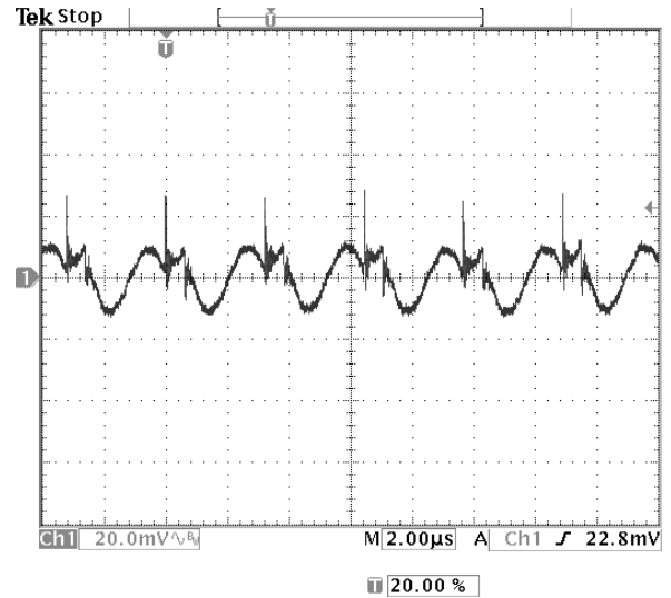
Fig-2.0V-5: Output voltage ripple (20mV/div.) for V_{out}=2.0V at full rated load current into a resistive load with external capacitance 47\mu F \times 2 ceramic + 1uF ceramic at V_{in}=12.0V . Time scale: 2 us/div
