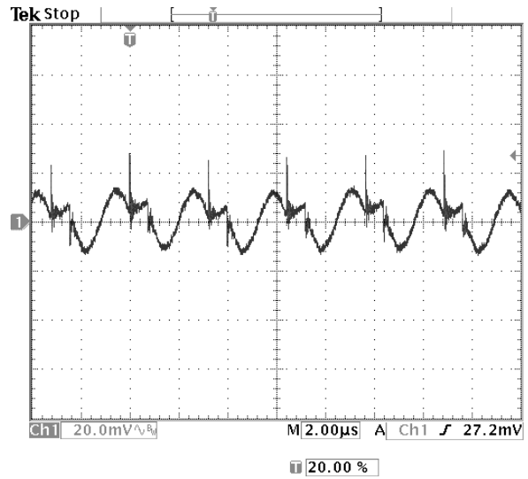
Fig-2.5V-5: Output voltage ripple (20mV/div.) for V_{out}=2.5V at full rated load current into a resistive load with external capacitance 47\mu F \times 2 ceramic + 1uF ceramic at V_{in}=12.0V . Time scale: 2 us/div
