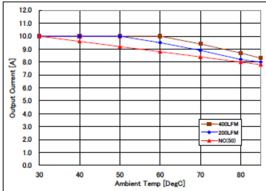
Fig-5.0V-1: Available load current vs. ambient temperature and airflow rates for Vout=5.0V with Vin=12.0V. Maximum component temperature \leq 120^{\circ}\text{C}
