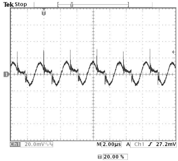
Fig-3.3V-5: Output voltage ripple (20mV/div.) for V_{out}=3.3V at full rated load current into a resistive load with external capacitance 47\mu F \times 2 ceramic + 1uF ceramic at V_{in}=12.0V . Time scale: 2 us/div
