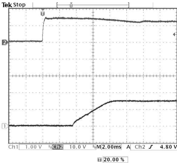
Fig-1.5V-4: Turn-on transient for V_{out}=1.5V with application of V_{in} at full rated load current (resistive) and 47\mu F \times 2 external capacitance at V_{in}=12.0V . Top trace: V_{in} (10V/div.) Bottom trace: output voltage (1V/div.) Time scale: 2 ms/div.
