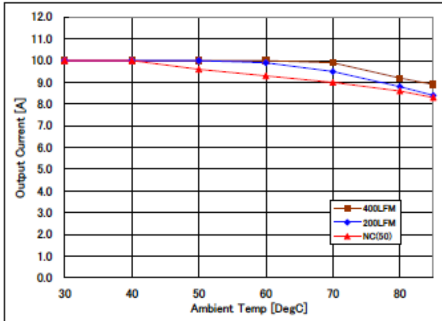
Fig-2.5V-1: Available load current vs. ambient temperature and airflow rates for Vout=2.5V with Vin=12.0V. Maximum component temperature ≤ 120°C
