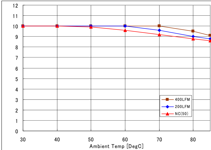
Fig-1.8V-1: Available load current vs. ambient temperature and airflow rates for Vout=1.8V with Vin=12.0V. Maximum component temperature \leq 120^{\circ}\text{C}
