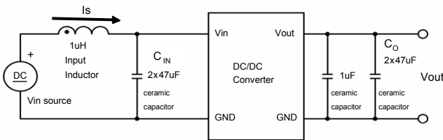
Fig. F: Test setup for measuring output voltage ripple
