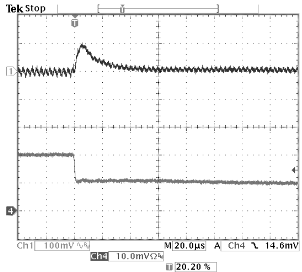
Fig-2.5V-7: Output voltage response for V_{out}=2.5V to positive load current step-change from 10A to 5A with slew rate of -5A/us at V_{in}=12.0V . C_o=47\mu F \times 2 ceramic. Top trace: output voltage (100mV/div.) Bottom trace: load current (5A/div.) Time scale: 20us/div.
