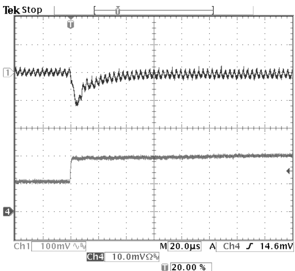
Fig-5.0V-6: Output voltage response for V_{out}=5.0V to positive load current step-change from 5A to 10A with slew rate of 5A/\mu s at V_{in}=12.0V . C_o=47\mu F \times 2 ceramic. Top trace: output voltage (100mV/div.) Bottom trace: load current (5A/div.) Time scale: 20us/div.
