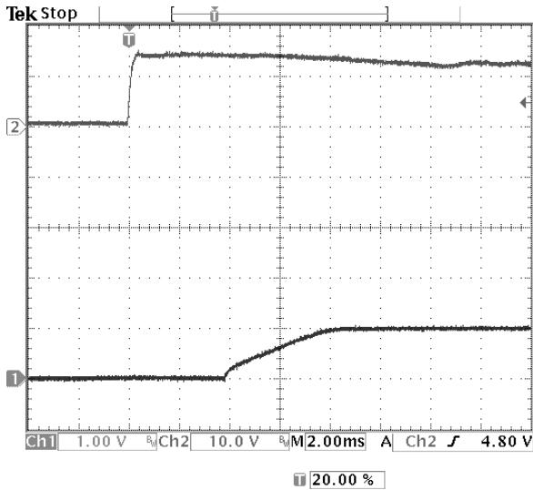
Fig-1.0V-4: Turn-on transient for V_{out}=1.0V with application of V_{in} at full rated load current (resistive) and 47\mu F \times 2 external capacitance at V_{in}=12.0V . Top trace: V_{in} (10V/div.) Bottom trace: output voltage (1V/div.) Time scale: 2 ms/div.
