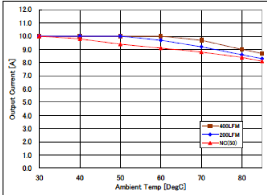
Fig-3.3V-1: Available load current vs. ambient temperature and airflow rates for V_{out}=3.3V with V_{in}=12.0V . Maximum component temperature \leq 120^{\circ}C
