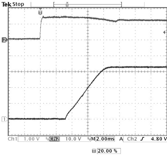
Fig-3.3V-4: Turn-on transient for V_{out}=3.3V with application of V_{in} at full rated load current (resistive) and 47\mu F \times 2 external capacitance at V_{in}=12.0V . Top trace: V_{in} (10V/div.) Bottom trace: output voltage (1V/div.) Time scale: 2 ms/div.
