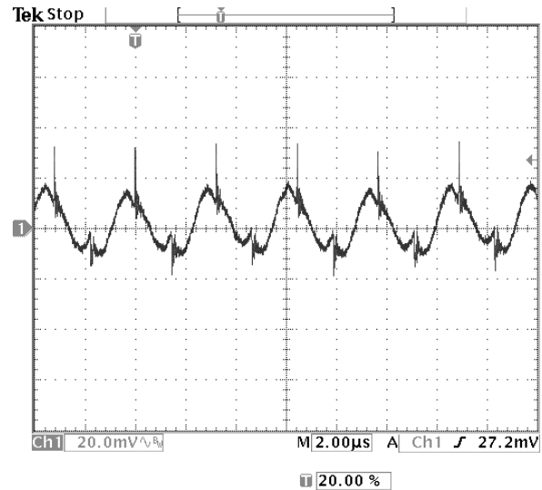
Fig-5.0V-5: Output voltage ripple (20mV/div.) for V_{out}=5.0V at full rated load current into a resistive load with external capacitance 47\mu F \times 2 ceramic + 1\mu F ceramic at V_{in}=12.0V . Time scale: 2 us/div
