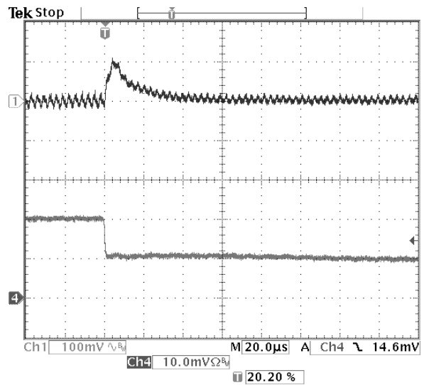
Fig-3.3V-7: Output voltage response for V_{out}=3.3V to positive load current step-change from 10A to 5A with slew rate of -5A/us at V_{in}=12.0V . C_o=47\mu F \times 2 ceramic. Top trace: output voltage (100mV/div.) Bottom trace: load current (5A/div.) Time scale: 20us/div.
