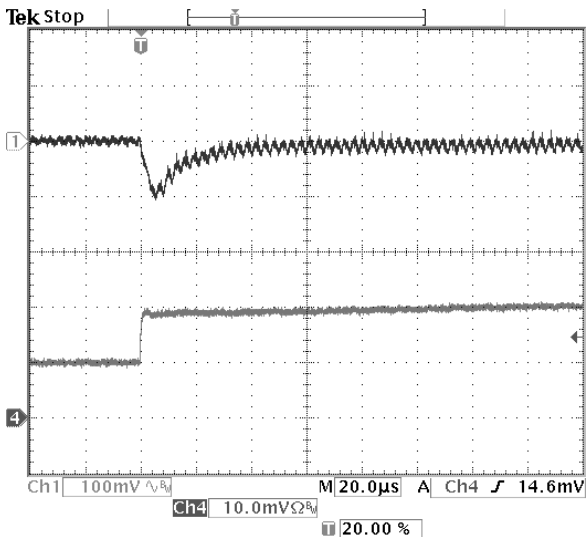
Fig-1.8V-6: Output voltage response for V_{out}=1.8V to positive load current step-change from 5A to 10A with slew rate of 5A/us at V_{in}=12.0V . C_o=47\mu F \times 2 ceramic. Top trace: output voltage (100mV/div.) Bottom trace: load current (5A/div.) Time scale: 20us/div.
