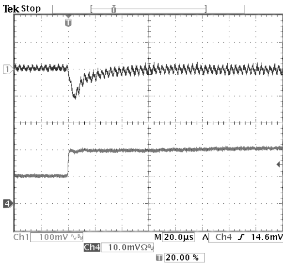
Fig-3.3V-6: Output voltage response for V_{out}=3.3V to positive load current step-change from 5A to 10A with slew rate of 5A/us at V_{in}=12.0V . C_o=47\mu F \times 2 ceramic. Top trace: output voltage (100mV/div.) Bottom trace: load current (5A/div.) Time scale: 20us/div.
