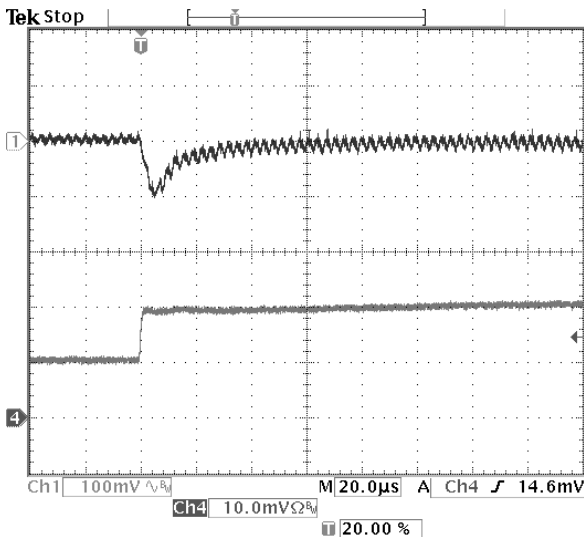
Fig-2.0V-6: Output voltage response for V_{out}=2.0V to positive load current step-change from 5A to 10A with slew rate of 5A/us at V_{in}=12.0V . C_o=47\mu F \times 2 ceramic. Top trace: output voltage (100mV/div.) Bottom trace: load current (5A/div.) Time scale: 20us/div.
