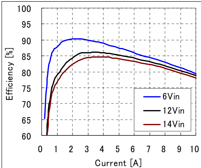
Fig-1.2V-2: Efficiency vs. load current and input voltage for Vout=1.2V. Airflow rate=200 LFM (1.0 m/s) and Ta=25°C.
