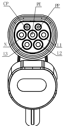
(Pin Layout Chart)
