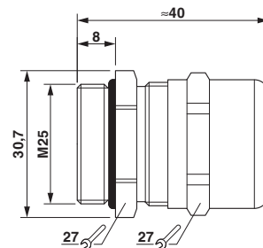
Dimensional drawing
