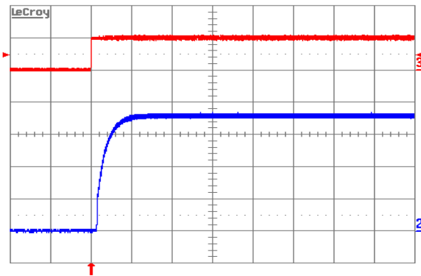
Figure 6. Turn-on transient at full rated load current (resistive) with C_o = 1 \mu\text{F cer} + 10 \mu\text{F tant} at V_{in} = 48 \text{ V} , triggered via ON/OFF pin. Top trace: ON/OFF signal (5 V/div.). Bottom trace: Output voltage (0.5 V/div.). Time scale: 5 ms/div.
