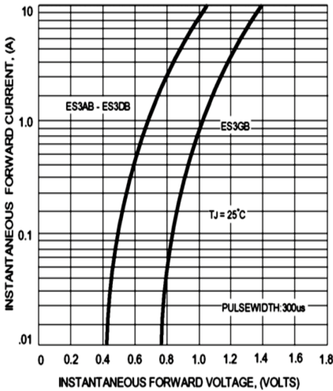
FIG.3 - TYPICAL FORWARD CHARACTERISTICS
