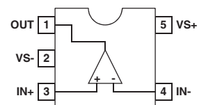
EL5193 (5 LD SOT-23) TOP VIEW
