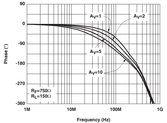
Non-Inverting Frequency Response (Phase) SO8 Package
