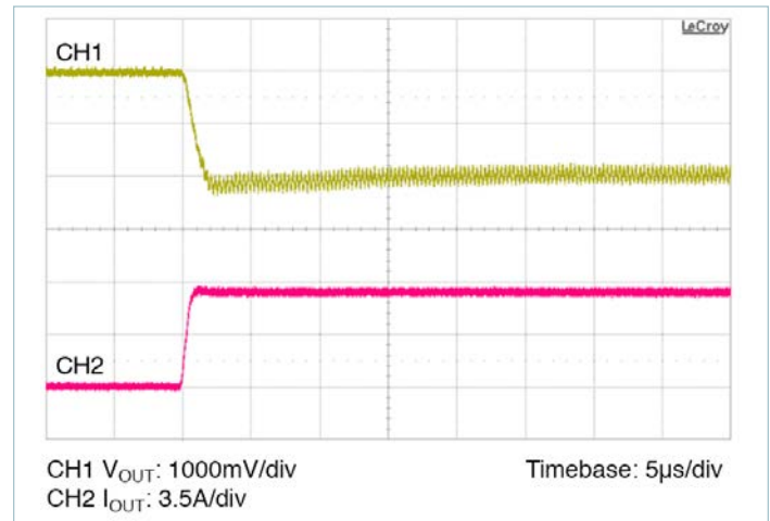
Figure 14 — 0A – Full load transient response: C_{IN} = 100\mu\text{F} , no external C_{OUT}
