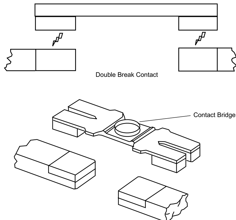
Figure 2 - Movable Contact
