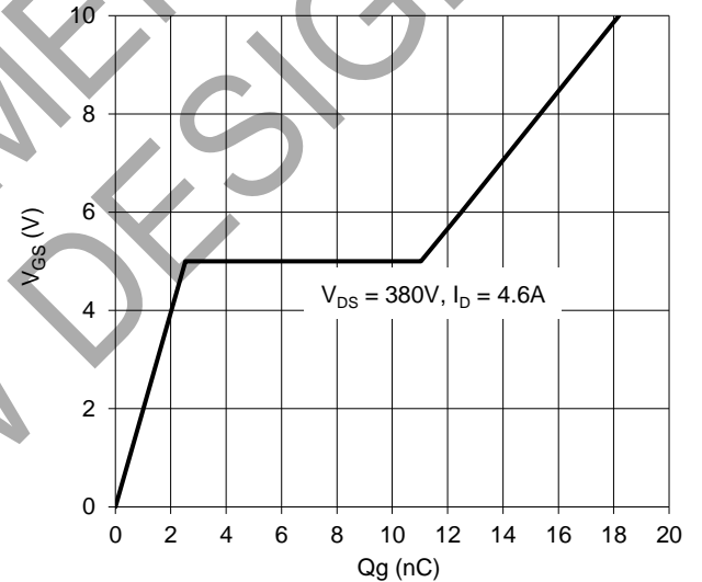
Figure 10. Gate Charge
