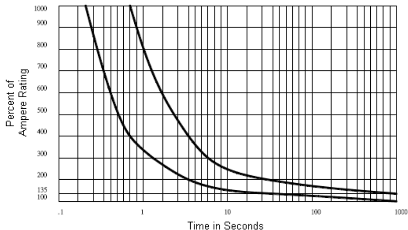
Part number: MRCBP4-PM Time Current Curves
