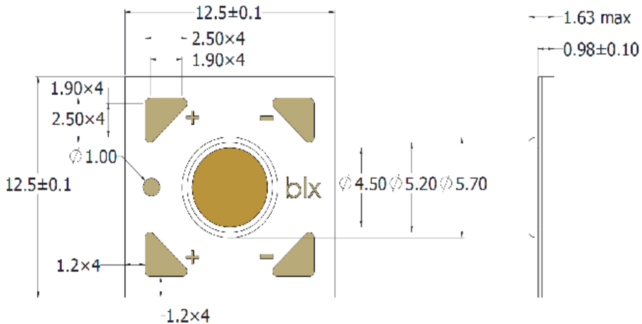
Figure 17: Drawing for V4 HD LED Array
