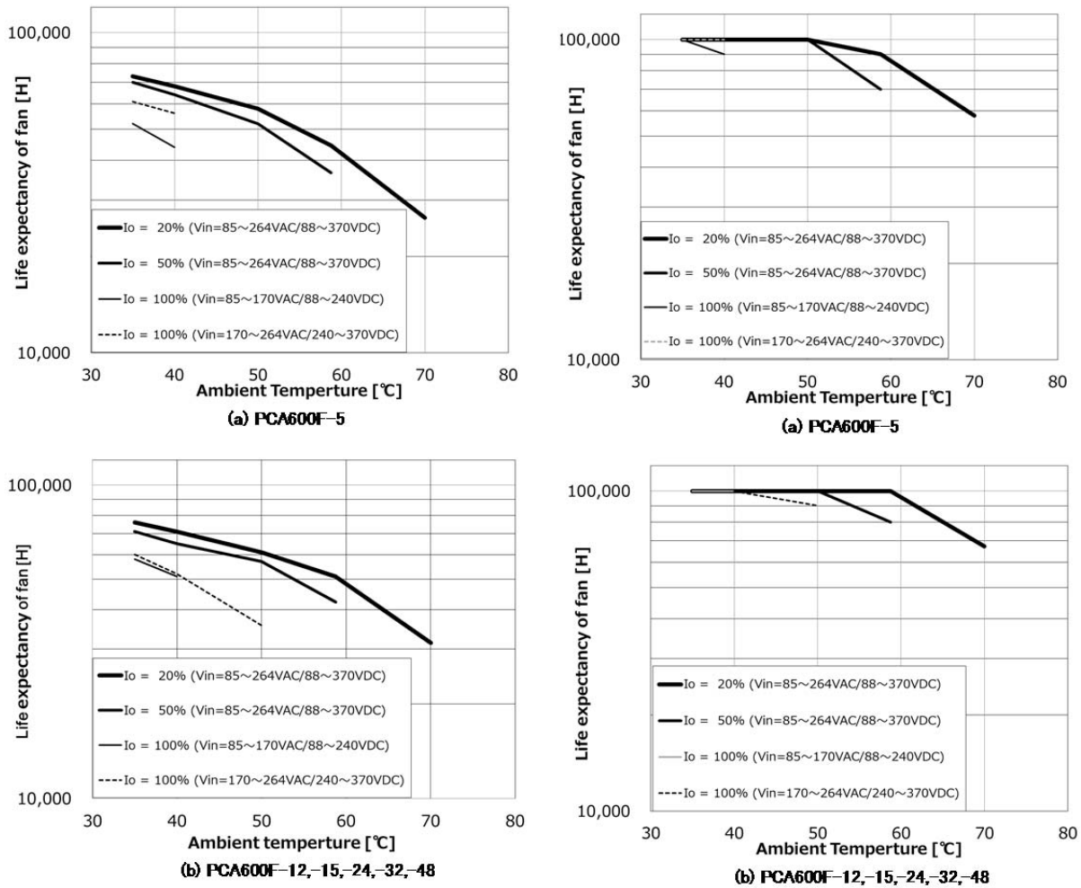
Fig. 2.2 Life expectancy of fan (Left : Current, Right : After Changed)
