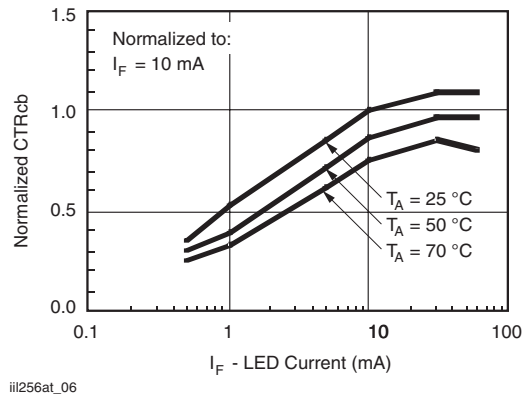
Figure 6. Normalized CTR_{cb}
