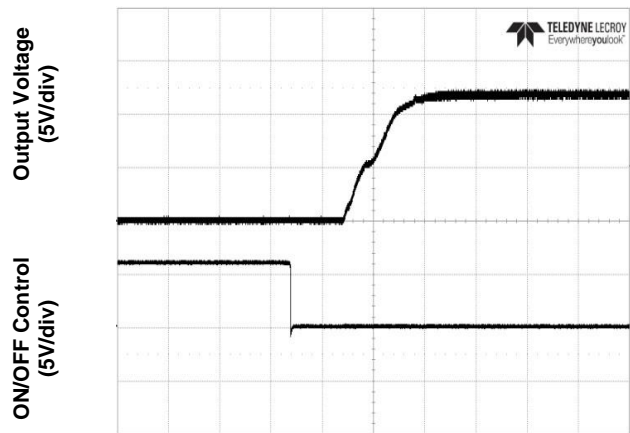
Figure 4. Start-Up from Enable Control (typical Vin, full load, 1,000µF external output capacitance)
