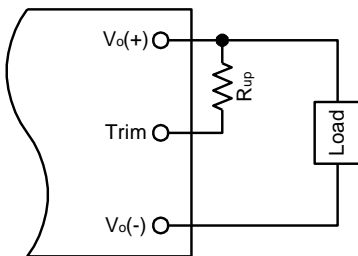
Figure 14. Circuit to Increase Output Voltage
