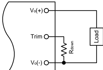
Figure 13. Circuit to Decrease Output Voltage
