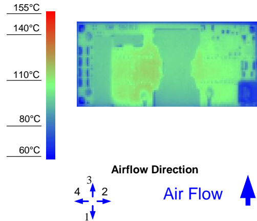
Figure 8. Thermal Image for Airflow Direction 3 (18A output, 55°C ambient, 200 LFM, typical Vin, open frame unit)
