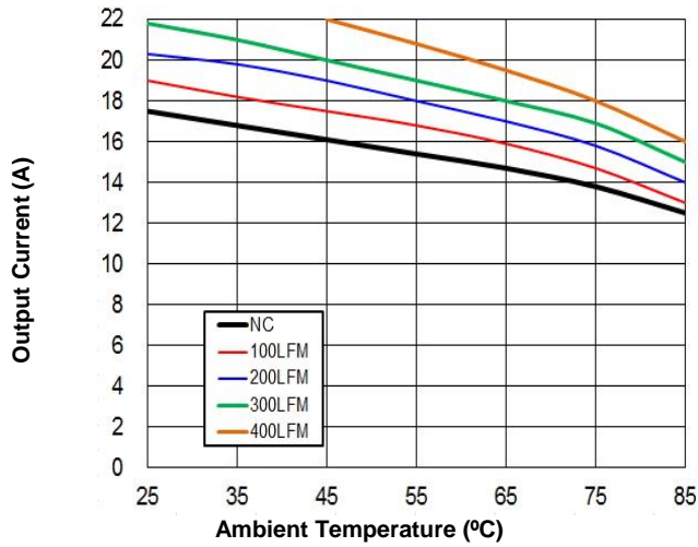
Figure 7. Current Derating Curve for Airflow Direction 3 (Ref. Fig. 8 for Airflow Direction; typical Vin, open frame unit)
