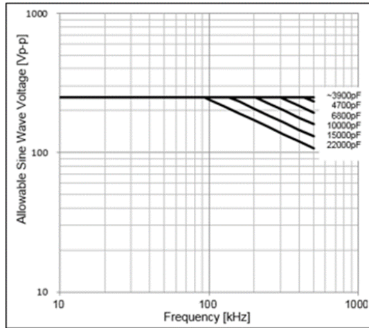
Chip(LxW): 3.2x1.6mm C0G(5C) Char. Rated Voltage:DC250V
