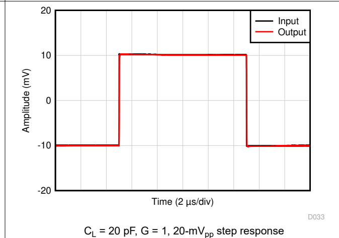
Figure 6-34. Small-Signal Step Response
