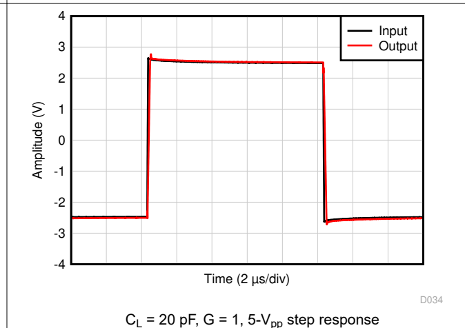
Figure 6-36. Large-Signal Step Response
