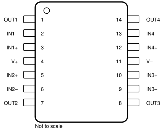
Not to scale Figure 5-4. TLV9164-Q1 D and PW Package, 14-Pin SOIC and TSSOP (Top View)
