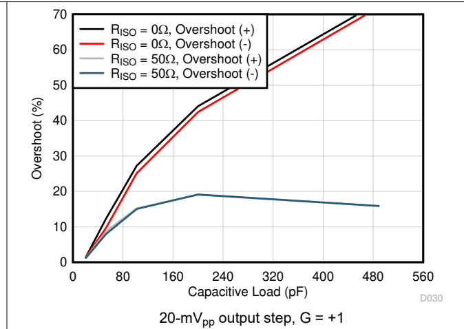
Figure 6-32. Small-Signal Overshoot vs Capacitive Load
