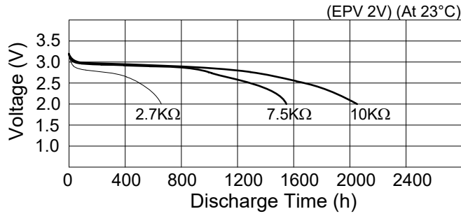
Figure 1. Discharge Characteristics
