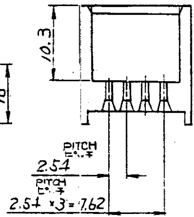
SECT "A-A"
